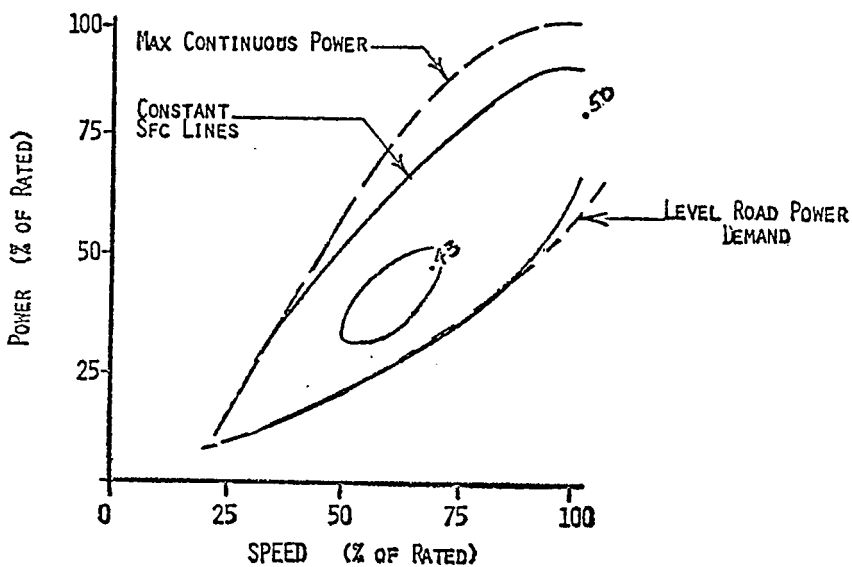
HYBRID ENGINE PART LOAD PERFORMANCE
