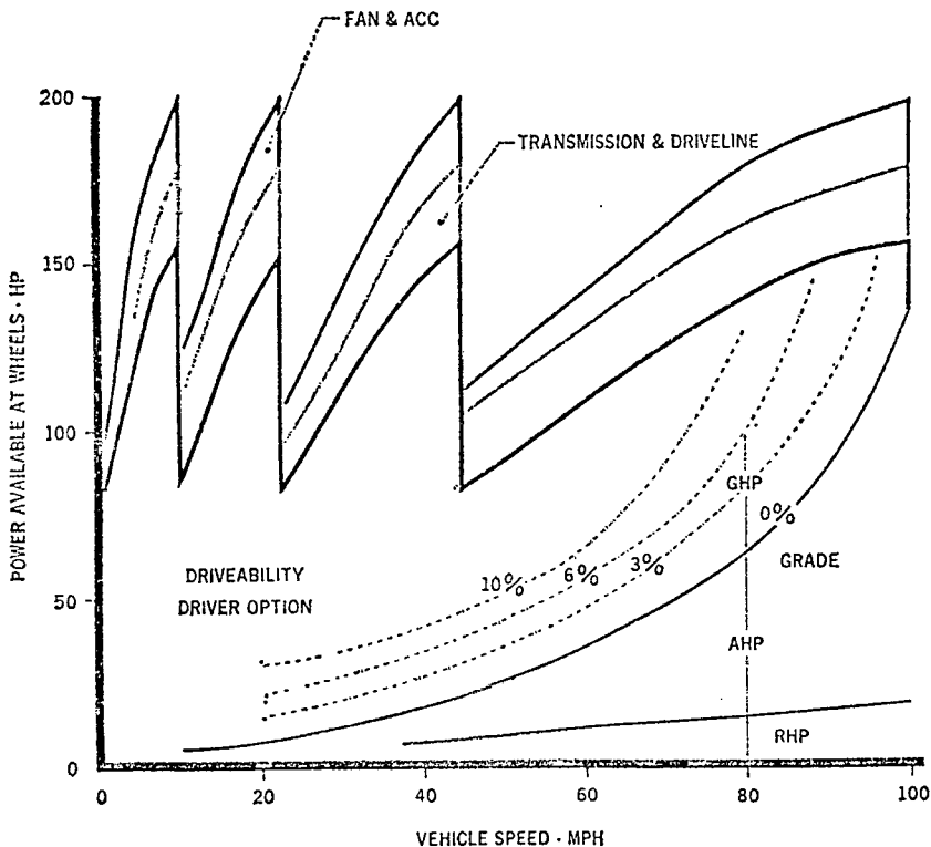
"REFERENCE AUTO" POWER - SPEED MAP
